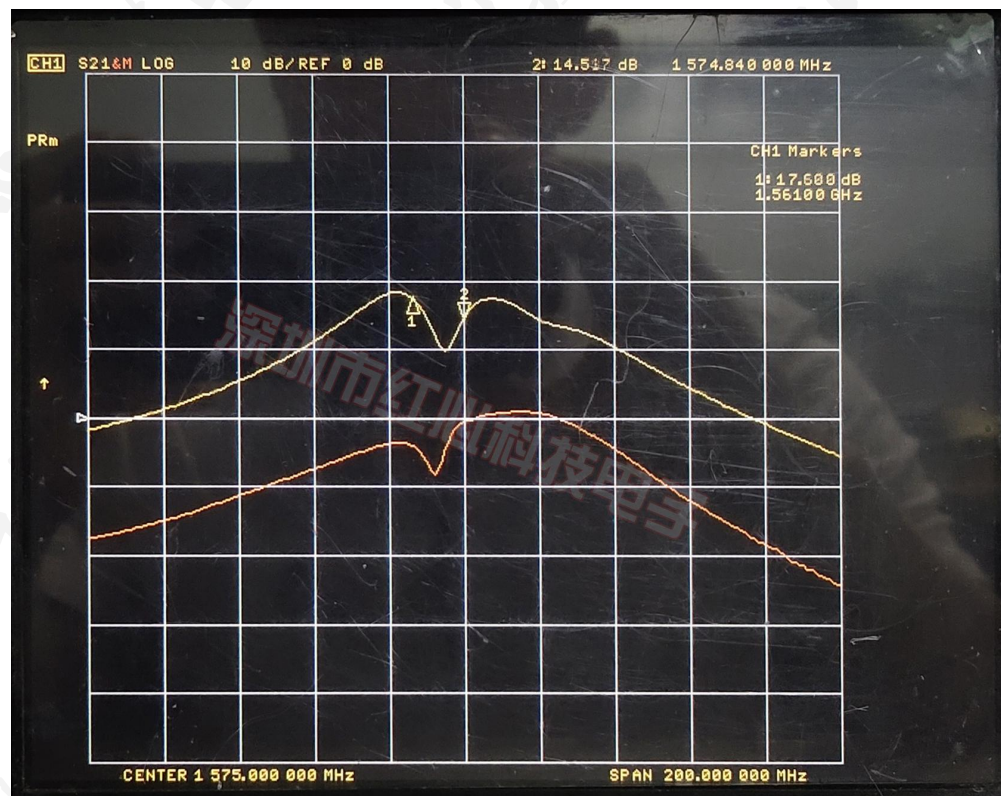
(Gain)增益图
